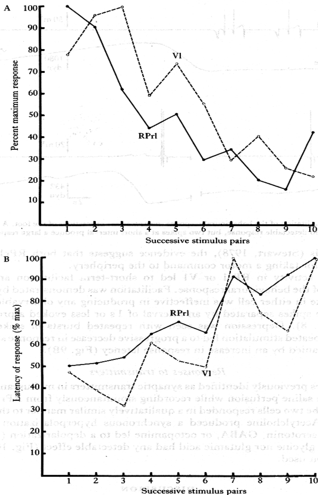
Fig. 9. Depression of the behavioural response. In separate experiments, RPr1 (solid line) and V1 (broken line) were stimulated intracellularly with depolarizing pulses (2 s) at 1 \text{ min}^{-1} . For RPr1, the number of spikes elicited by each stimulus was constant within the range 8–10; for V1, the number of spikes per stimulus increased about 30% during the series of trials. The graphs show data which has been pooled from successive stimulus pairs. (A) Amplitude of foot contractions. (B) Latency of foot contractions measured from the first spike in the evoked train of spikes.
