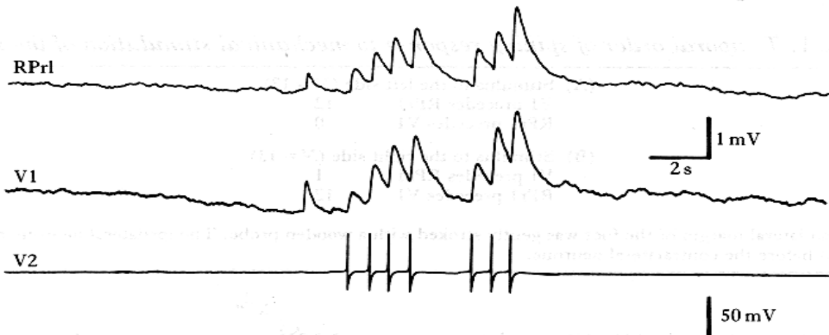
Fig. 6. Intrasomatic stimulation of cell V2 leads to parallel facilitation of EPSPs in RPr1 and V1. High frequency filtration was employed in recording the postsynaptic responses.
