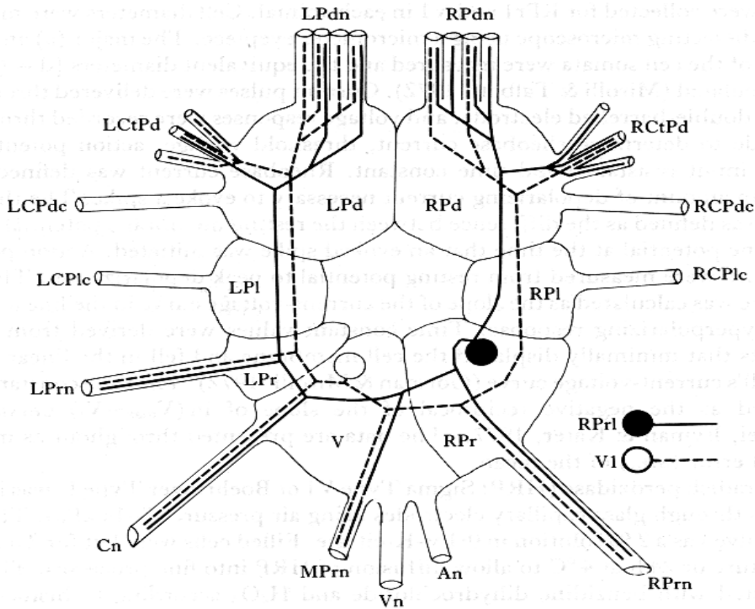
Fig. 1. Schematic representation of the dorsal aspect of the suboesophageal ganglionic ring (unfolded) in Achatina fulica . RPr1 projections are represented by solid lines. V1 projections are represented by broken lines. The axons of each cell coincide in all nerves except the pedal nerves, where the ipsilateral cell is numerically favoured. The number and arrangement of the pedal nerves has been simplified for purposes of clarity. Abbreviations: Pd, pedal; Pl, pleural; Pr, parietal; V, visceral; An, anal nerve; Cn, columellar nerve; CPdc, cerebropedal connective; CPlc, cerebropleural connective, CtPd, cutaneous pedal nerves. Also: R, right; L, left; M, medial; n, nerve.
