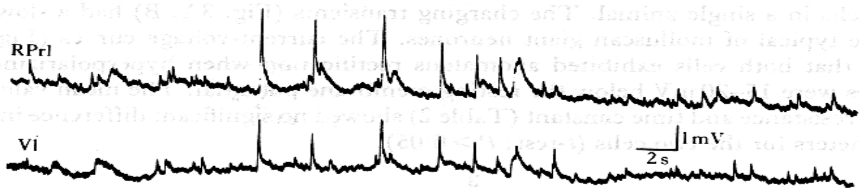
Fig. 4. Spontaneous synaptic inputs recorded simultaneously in RPr1 and V1. With few exceptions, EPSPs are synchronous in the two cells.
