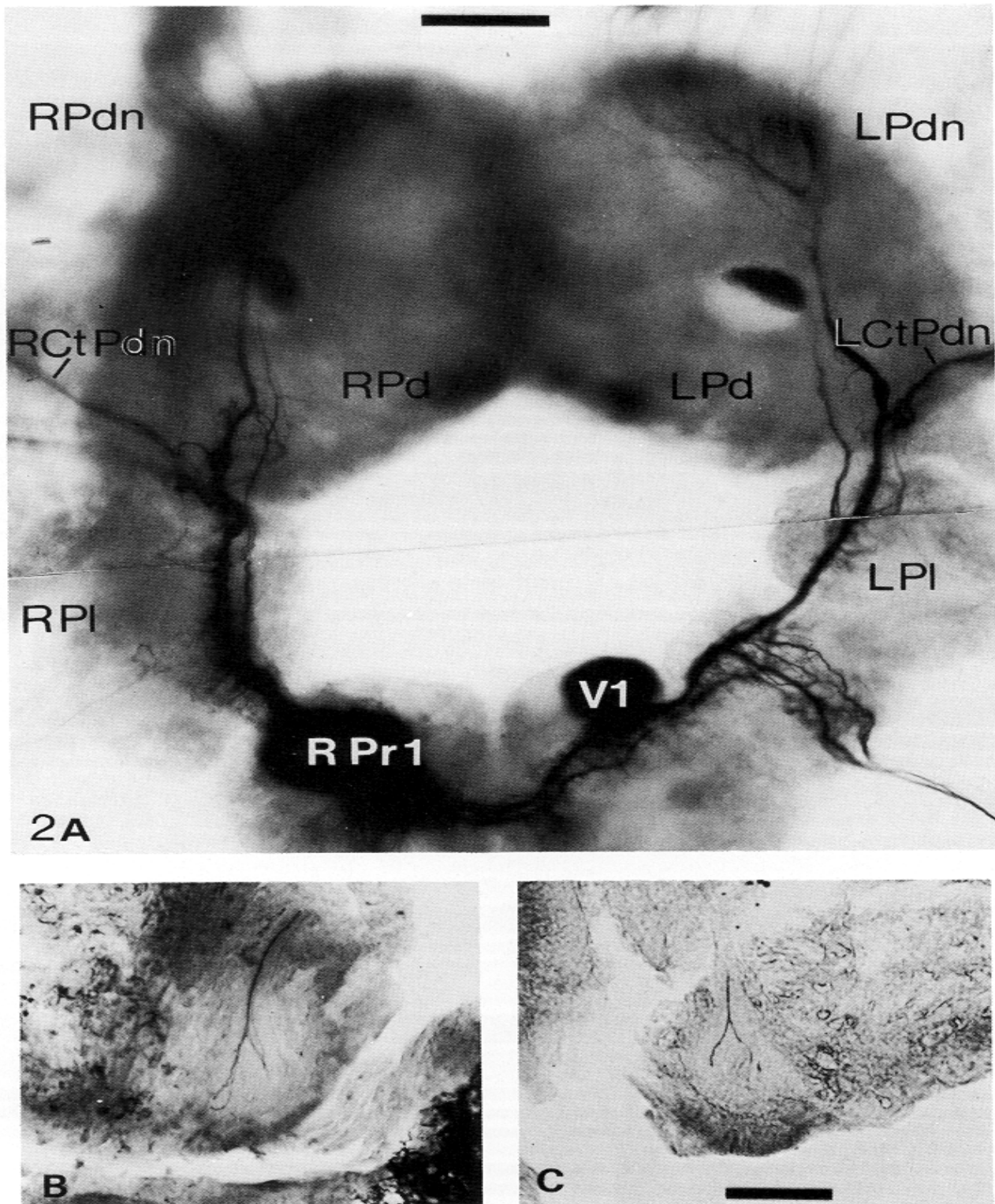
Fig. 2. (A) Morphological symmetry of RPr1 and V1 as revealed by intracellular injections of HRP. The figure is a composite of two photographs showing the ventral aspect of the suboesophageal ganglionic ring. Note the left-right reversal compared to Fig. 1. The statocysts are visible in the pedal ganglia. The thick process on each side belongs to the ipsilateral cell; the thin process belongs to the contralateral cell. Abbreviations as in Fig. 1. (B), (C) Sections through the mantle showing peripheral branches and presumed terminal sites of V1 axon (B) and RPr1 axon (C). (B) and (C) are taken from different animals. In both cases, the filled processes were followed from projections in the right parietal nerve. The magnification of (B) and (C) is the same. Scale bars: A = 300 \mu m; B, C = 100 \mu m.
