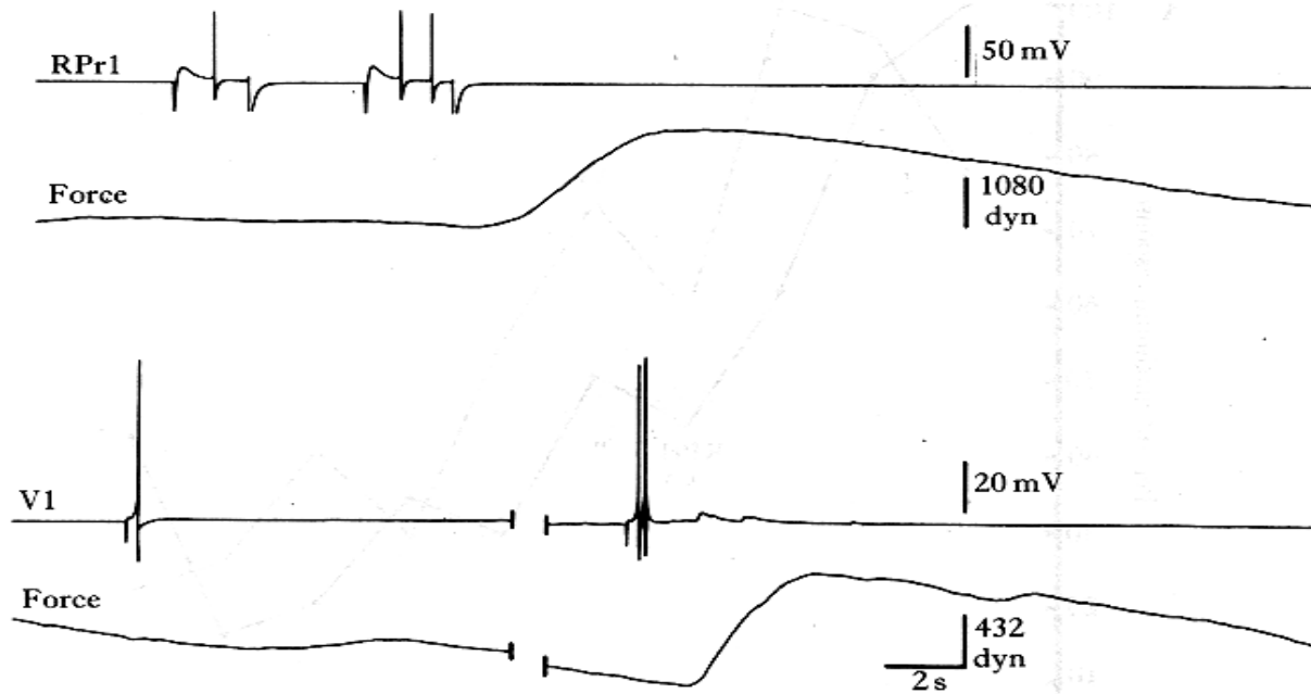
Fig. 8. Facilitation of the behavioural response, measured as contractions of the foot. A single spike produces no detectable response, but two spikes at a short interval produce a large response.
