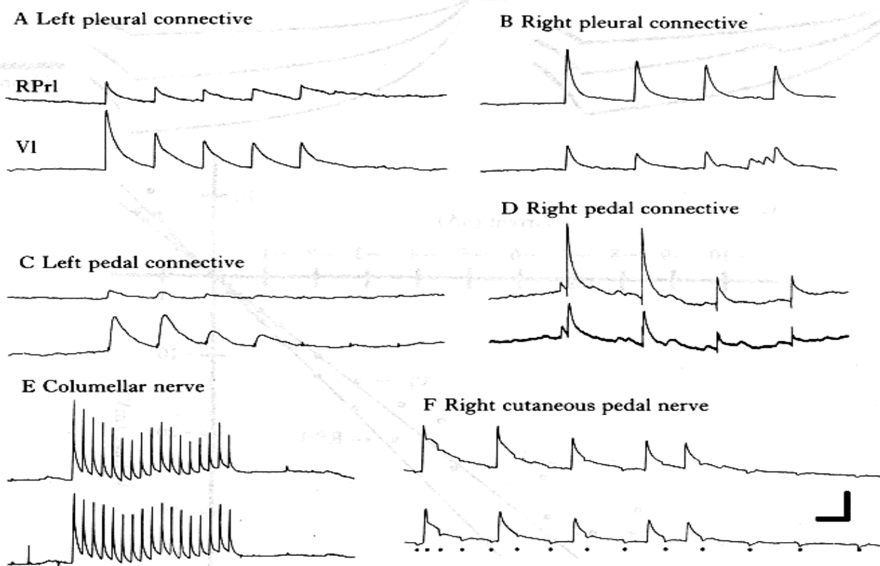
Fig. 5. Electrical stimulation of nerves and connectives. Repeated pulses (0.5 ms) were delivered through suction electrodes. Cellular responses are compound EPSPs. Note that when homologous connectives were stimulated independently on the right and left sides (A, B and C, D), the cell ipsilateral to the site of stimulation consistently produced the largest response. Depression of the response occurs in all cases. (E) Slow time scale shows that trial-to-trial variations in relative EPSP amplitude are closely matched in the two cells. (F) Synchronous IPSPs (marked by dots), as well as EPSPs, following stimulation of a cutaneous pedal nerve. IPSPs continue after termination of stimulus. Calibration scales are: A–D, 3 mV, 2 s; E, 7.5 mV, 10 s; F, 7.5 mV, 2 s.
