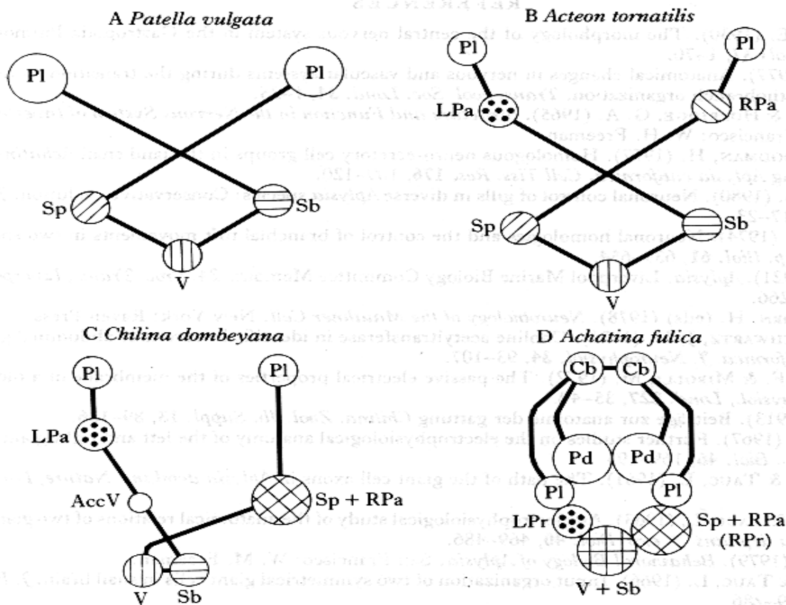
Fig. 11. Organization of the central nervous system (posterior portion) in gastropod molluscs. The examples show contemporary species that are considered (by the cited authors) to represent successive stages in the evolution of the pulmonate nervous system. (A) A prosobranch gastropod (Bargmann, 1930). (B) A primitive opisthobranch (Brace, 1977). (C) A primitive pulmonate (Haeckel, 1913). (D) An advanced pulmonate and the subject of the present study. The fusion of ganglia is indicated by cross-hatching. Abbreviations: AccV, accessory visceral ganglion; Cb, cerebral ganglion; Pa, pallial ganglion; Pd, pedal ganglion; Pl, pleural ganglion; Pr, parietal ganglion; Sp, suprainstestinal ganglion; V, visceral ganglion; L, left; R, right.
